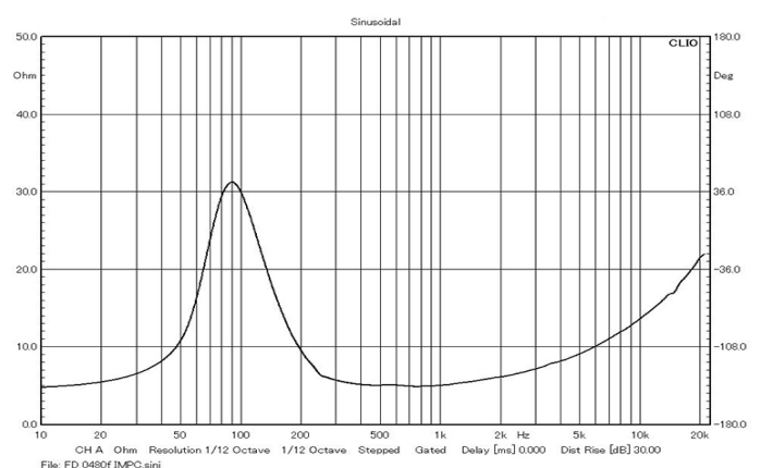
Impedance curve of FD 4080f
